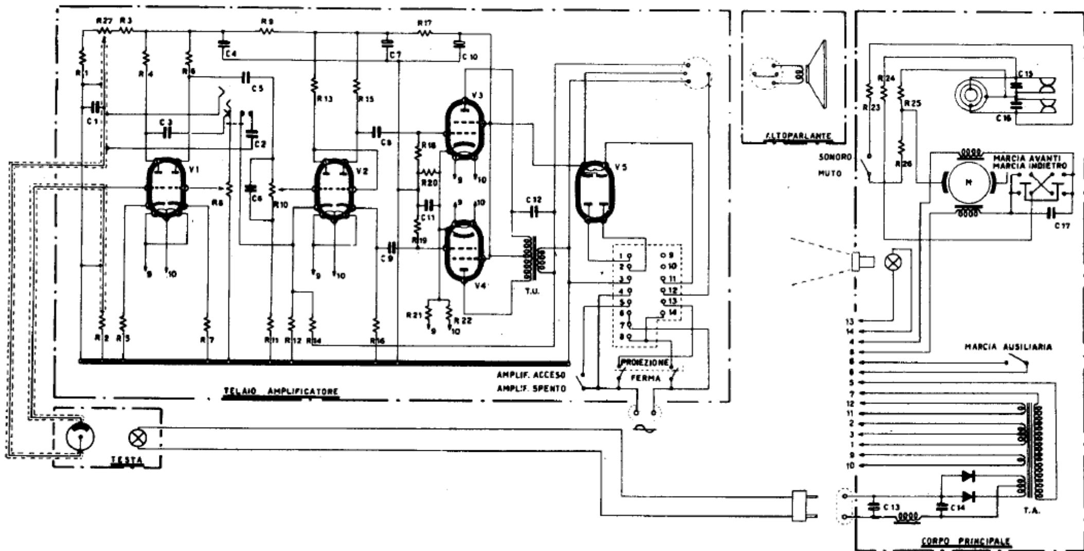
Ducati RG2504-4 Amplifier
